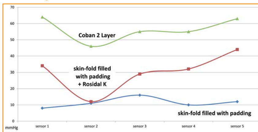
Figure 11: Pressure profile of the materials under investigation on the artificial leg with the skinfold
