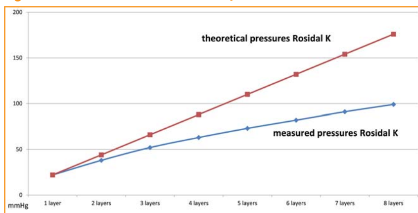
Figure 3: Theoretical and measured pressure values of Rosidal K®
